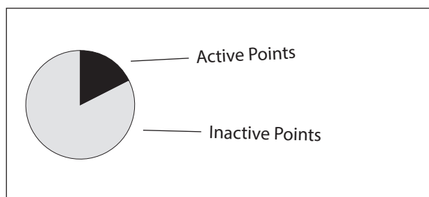
Figure 05 – Ratio between active and inactive point in Brazil in march/2017
